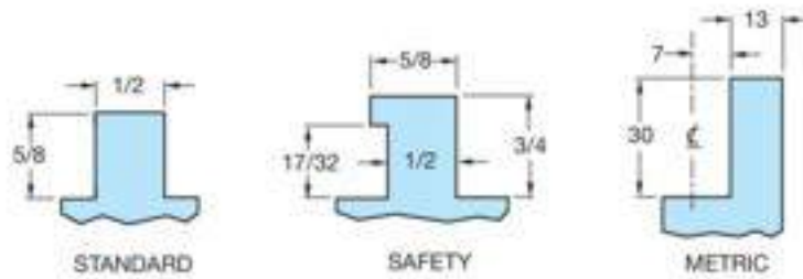
Common types of brake die tongues - others on request
